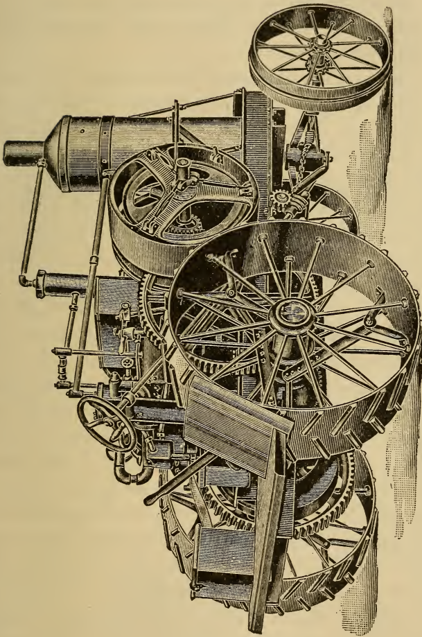
FIG. 63.—HART-PARR GASOLINE TRACTION ENGINE.
